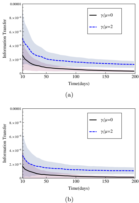
FIG. 2: Mean and std for the estimate of information transfer averaging over 200 pairs of users with \gamma/\mu = 0, 2 as a function of time. (a) Results without correcting for bias and (b) with Panzeri-Treves bias correction[12].
