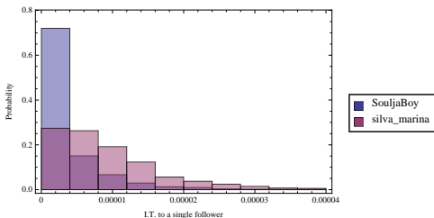
FIG. 11: A histogram showing the probability distribution of outgoing transfer entropy for followers of two different Twitter accounts.
