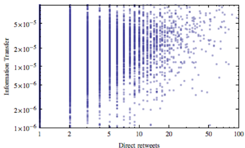
FIG. 9: The number of URLs that were first tweeted by user X and subsequently tweeted by X 's follower, Y , is correlated with the calculated transfer entropy between X and Y , even though transfer entropy is calculated only from the timing of activity, without regard for specific URLs. Pearson's correlation coefficient is 0.22.
