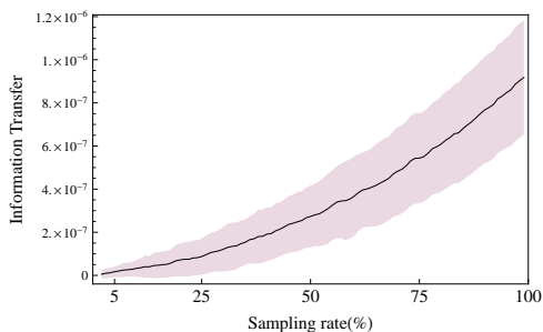
FIG. 3: A summary of the mean and std of the inferred value of T_{Y \rightarrow X} averaged over 200 trials as a function of the sampling rate, with T = 500 days and \gamma/\mu = 2 .
