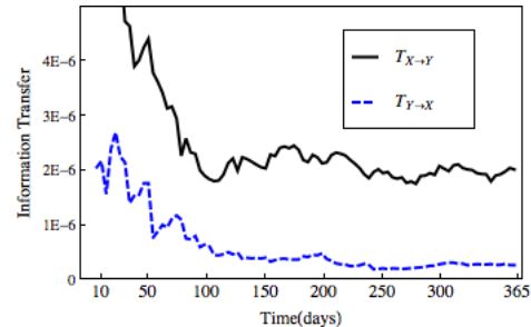
FIG. 1: If we have influence from X \rightarrow Y but not vice versa, the asymmetry in the information transfer correctly reflects the direction of influence. Information transfer plotted for a single pair of users.
