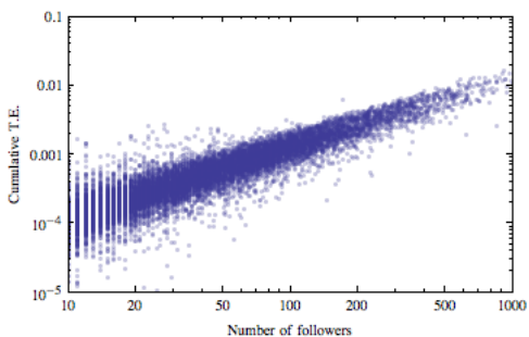
FIG. 8: For each user, we compare the number of their followers to their cumulative outgoing transfer entropy. Note that the outgoing transfer entropy may differ by an order of magnitude for people with the same number of followers.
