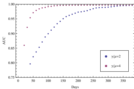
FIG. 6: AUC of the network inferred using transfer entropy as a function of T , with \gamma/\mu = 2, 4 .
